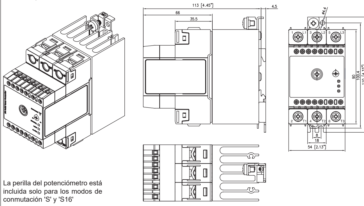
RGC2..I25, RGC2..V25 RGC3..I20, RGC3..V20
