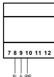
Fig. 9 Port RS485
