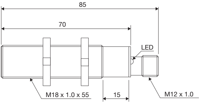
Fig. 8 Conector CA18CAF...M1IO
