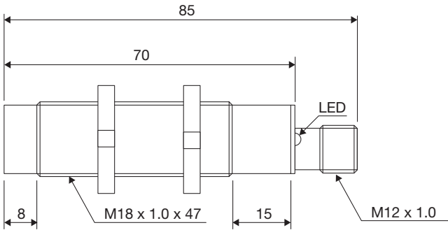
Fig. 9 Conector CA18CAN...M1IO
