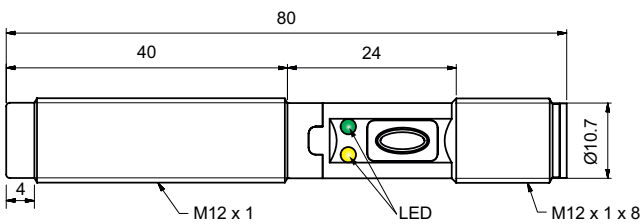
Fig. 9 Conector CA18EAN...M1IO
