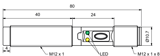
Fig. 9 Conector CA18CAN...M1IO
