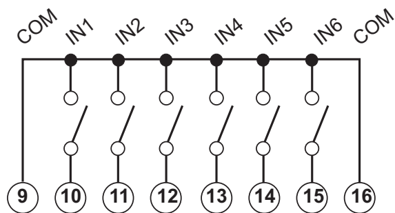
Fig. 24 MF 16 O6. 6 digital inputs and 6 static outputs
