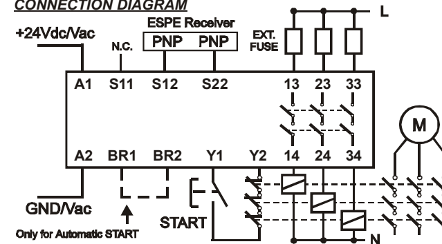
CONNECTION DIAGRAM
